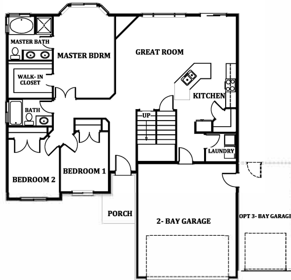
MAIN LEVEL
